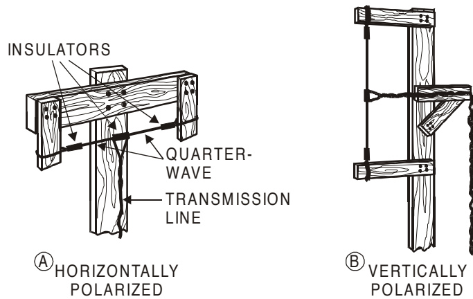
Figure O-7. Center-Fed Half-Wave Antenna.
